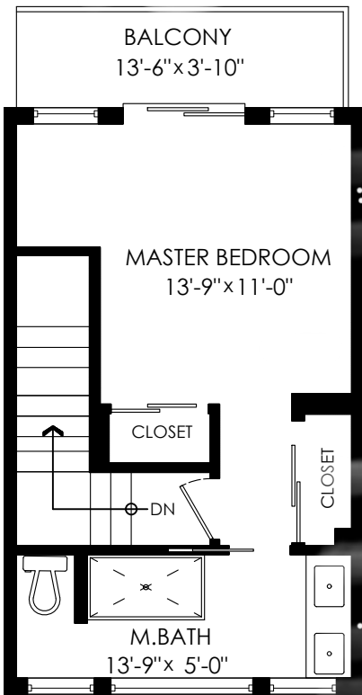
Top Floor Plan Floor Area: 355 sq.ft. Vault Ceiling Height: 11'-5"
