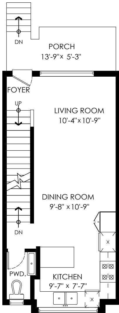
Main Floor Plan Floor Area: 443 sq.ft. Ceiling Height: 9'
