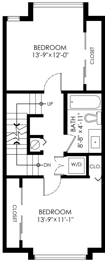
Upper Floor Plan Floor Area: 529 sq.ft. Ceiling Height: 8'
