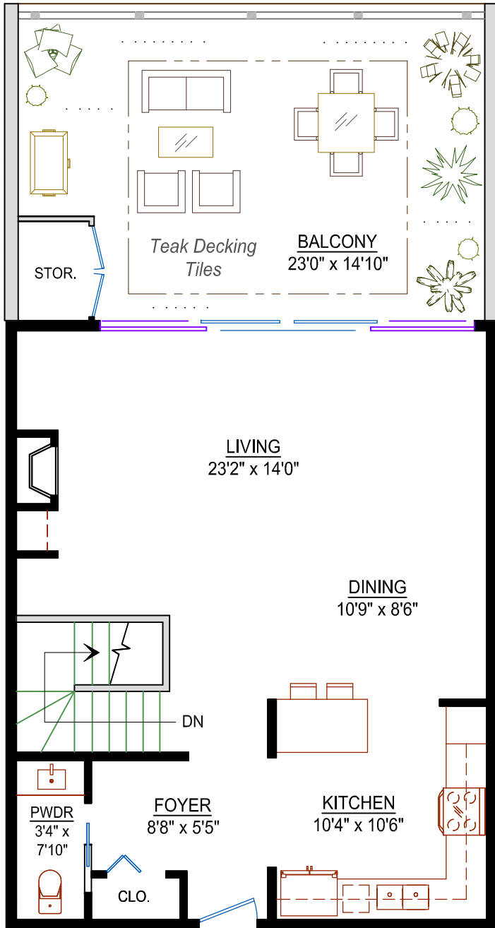
MAIN LEVEL Area: 711 sq. ft.
