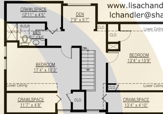
UPPER FLOOR PLAN FLOOR AREA: *718 sq.ft.
