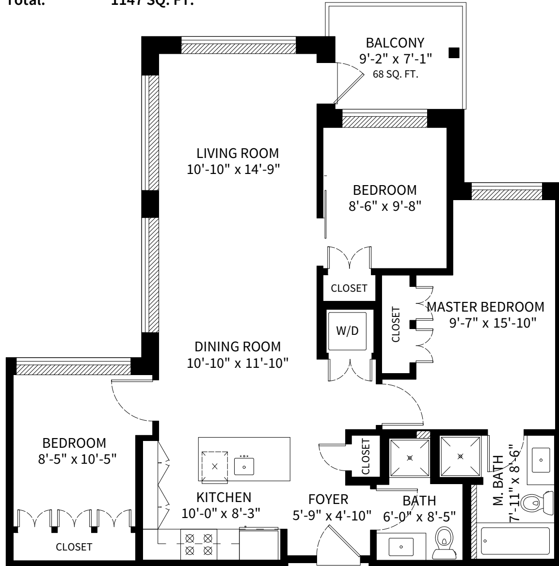
FLOOR PLAN Ceiling Height: 8'-11"
