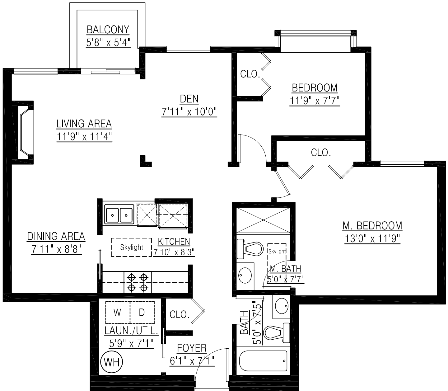
MAIN FLOOR PLAN FLOOR AREA: 960 sq.ft.
