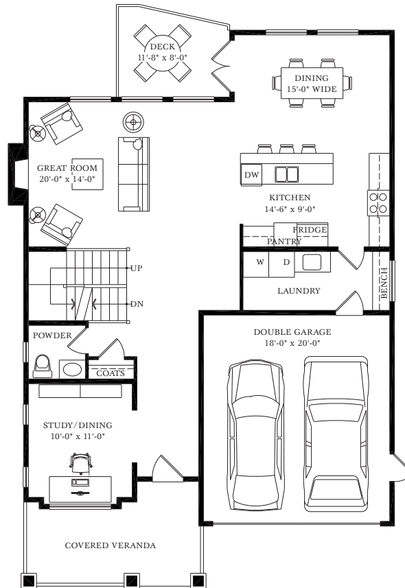
MAIN FLOOR
