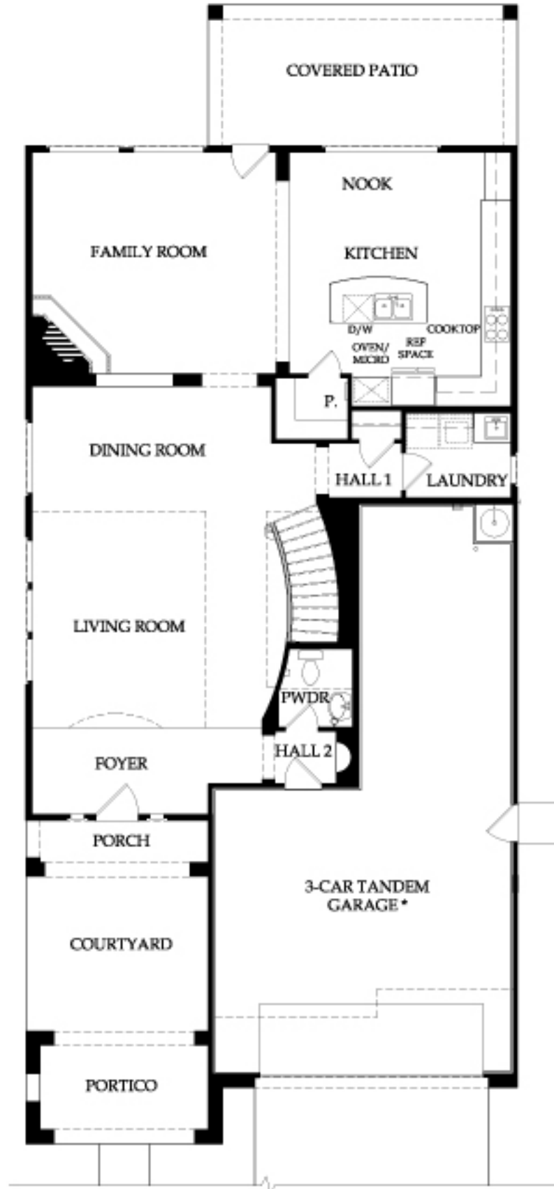
ELEVATION 'A' First Floor
