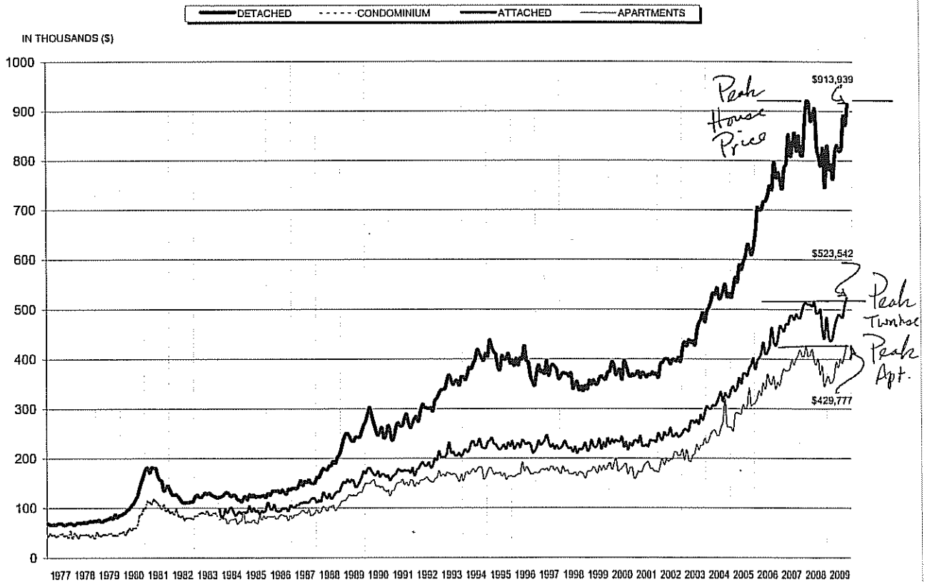
Real Estate Board of Greater Vancouver Average Price Graph January 1977 to October 2009
