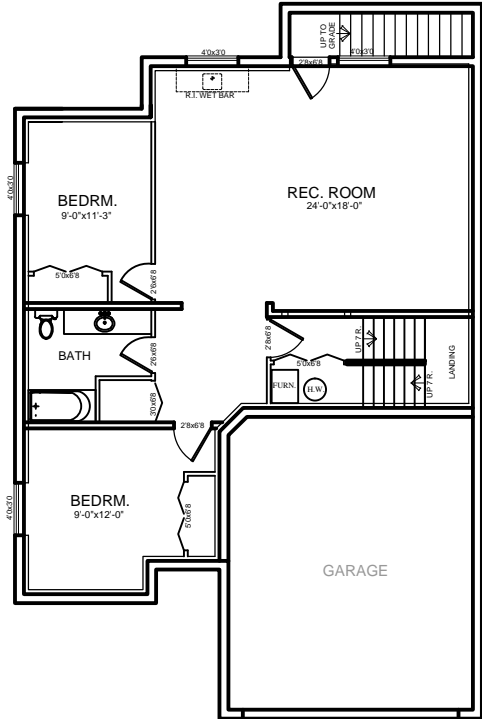
BASEMENT = 1122 SQ. FT.
