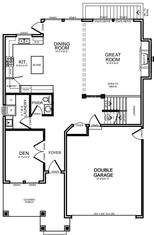
MAIN FLOOR = 1122 SQ. FT.
