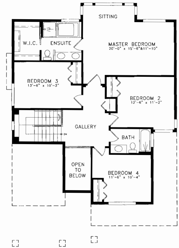
UPPER FLOOR PLAN: 1127 SQ. FT.
