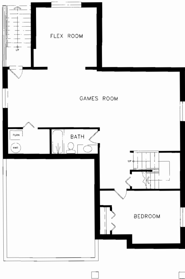
BASEMENT FLOOR PLAN: 1157 SQ. FT. (SHOWING OPTIONAL FINISHED BASEMENT. WALKOUT, WINDOWS & DOORS MAY VARY.)
