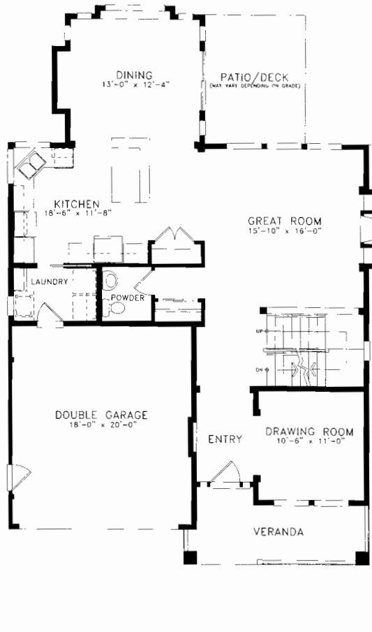
MAIN FLOOR PLAN: 1164 SQ.FT. GARAGE: 378 SQ. FT. VERANDA: 118 SQ. FT.
