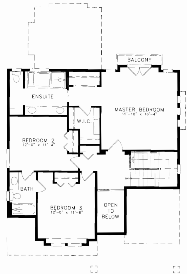
UPPER FLOOR PLAN: 1011 SQ.FT. BALCONY: 18 SQ. FT.
