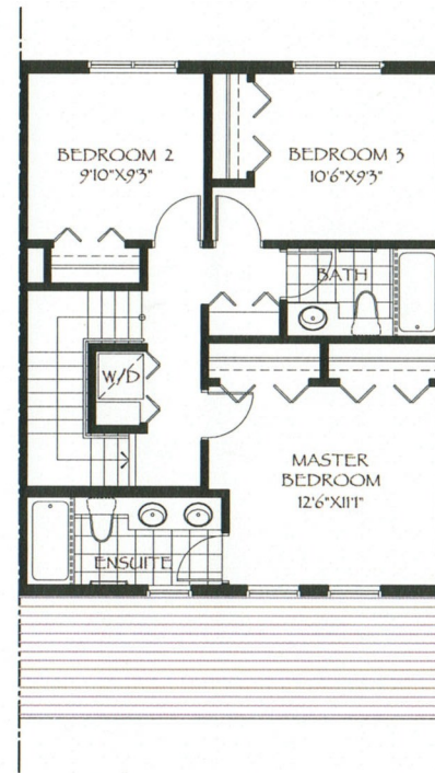
SECOND FLOOR PLAN 706 SQ.FT.
