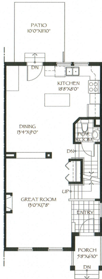
GROUND FLOOR PLAN 724 SQ.FT.
